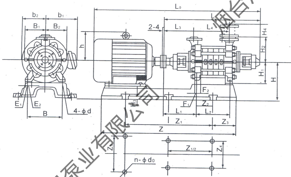
外形安装尺寸图 Overall and Installation Dimension
